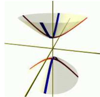
HYPERBOLOID II
