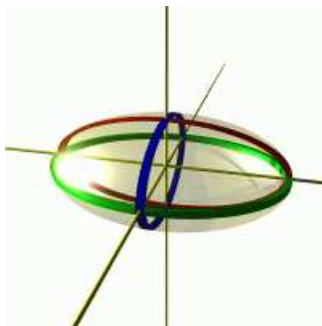
ELLIPSOID
