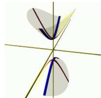
DEFORMED HYPERBOLOID
