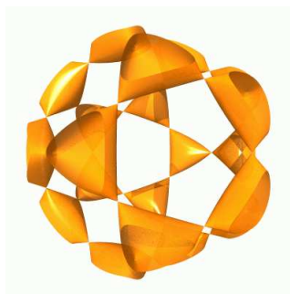
SEXTIC
