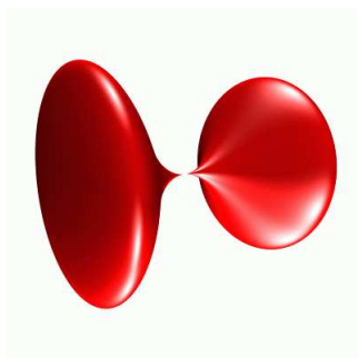
QUARTIC
