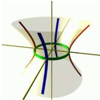
HYPERBOLOID I
