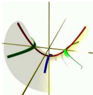
HYPERBOLIC PARABOLOID
