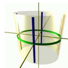
CYLINDER
