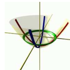
PARABOLOID
