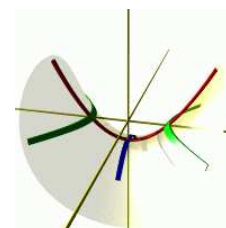
HYPERBOLIC PARABOLOID
