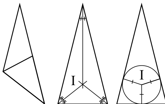
Figure 3.7: The incenter and the incircle.
