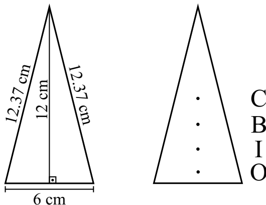
Figure 3.8: Isosceles triangle and its centers.
