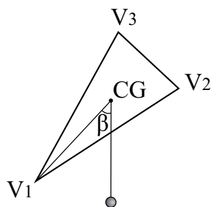
Figure 4.42: The vertical triangle supported at its barycenter will remain in equilibrium after release from rest for any angle \beta .
