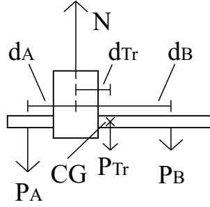
Figure 8.10: Conditions of equilibrium for an asymmetrical lever.
