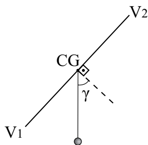
Figure 4.43: The inclined triangle supported by its barycenter remains in equilibrium for any angle \gamma .
