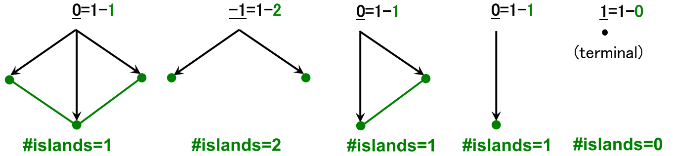
FIGURE 5. The rule for Poincare–Hopf index ( =1 - \text{\#destinations} ) for all eight patterns of downward connections. As there are three downward edges, the existence or absence of each edge results in eight patterns in total. However, to save space, the symmetric and equivalent three patterns were omitted. The green dots and edges represent the destinations called exit sets. The green integers denote the numbers of isolated destinations. The underlined integers denote the Poincare–Hopf indices for each top point. Note that the number of destinations is one and thus the index is zero except for the two patterns shown in Figure 3.
