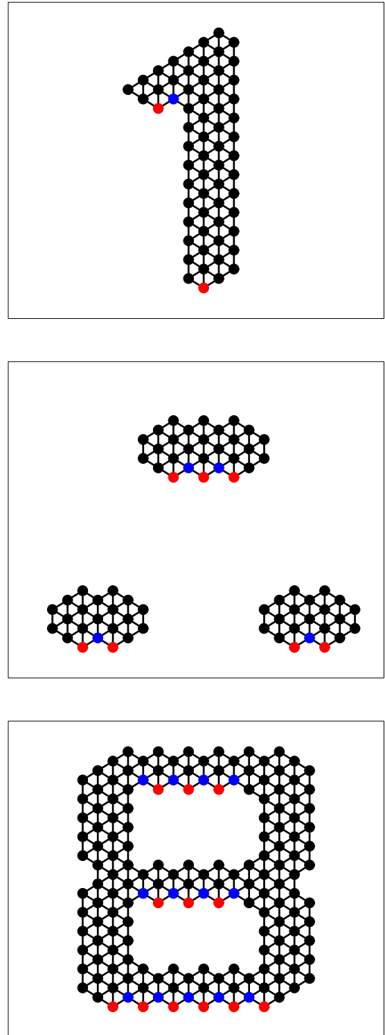
FIGURE 4. Additional examples of Poincaré-Hopf indices. The nonzero indices +1 and -1 were indicated by red and blue colors, respectively. The Euler characteristics via the Poincaré-Hopf index ( =\#red\ points - \#blue\ points ) is equal to the topological Euler characteristics ( =\#islands - \#holes ) for each case, that is, 1 , 3 , and -1 , respectively.
