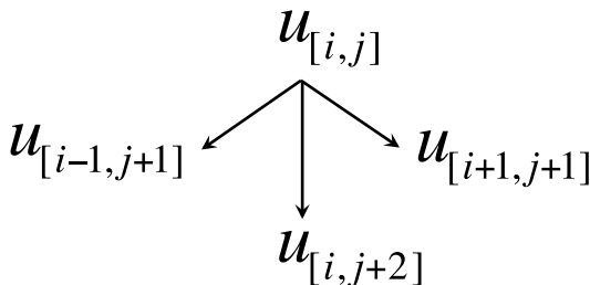
FIGURE 6. Notation to derive a logical operation for Poincare–Hopf index for downsampled case. As we downsample from a square lattice u_{[i,j]} to obtain a triangular lattice, we only consider the points where i+j is even and let u_{[i,j]} = 0 for i+j odd.
