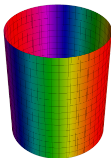
x^2 + y^2 = 1 Cylinder
