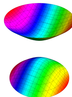
x^2 + y^2 - z^2 = -1 Two sheeted Hyperboloid
