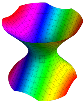
x^2 + y^2 - z^2 = 1 One sheeted Hyperboloid
