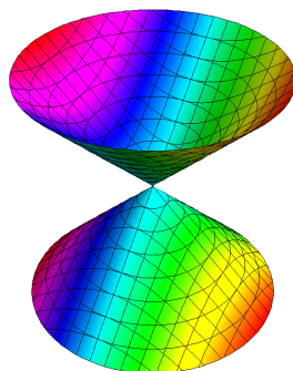
x^2 + y^2 - z^2 = 0 Cone
