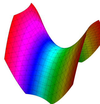
x^2 - y^2 - z = 0 Hyperbolic Paraboloid
