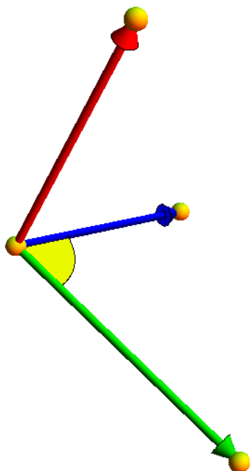
FIGURE 1. The cross product gives vectors perpendicular to both arguments. The length of the product is the area of the parallelogram.
