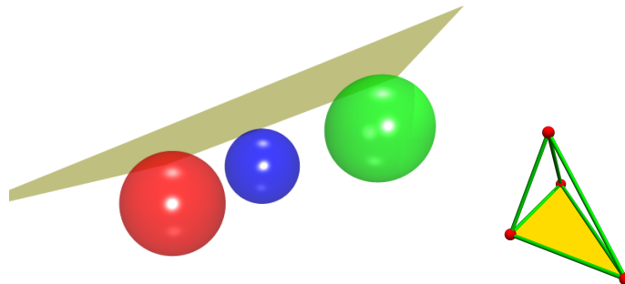
FIGURE 2. The sphere problem and the tetrahedron.
